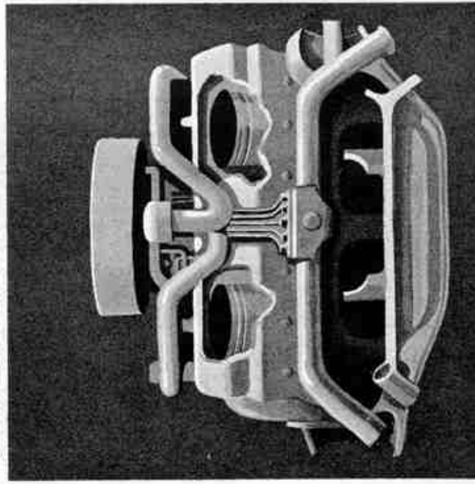
CROSS-SECTION OF POWER BOAT ENGINE
