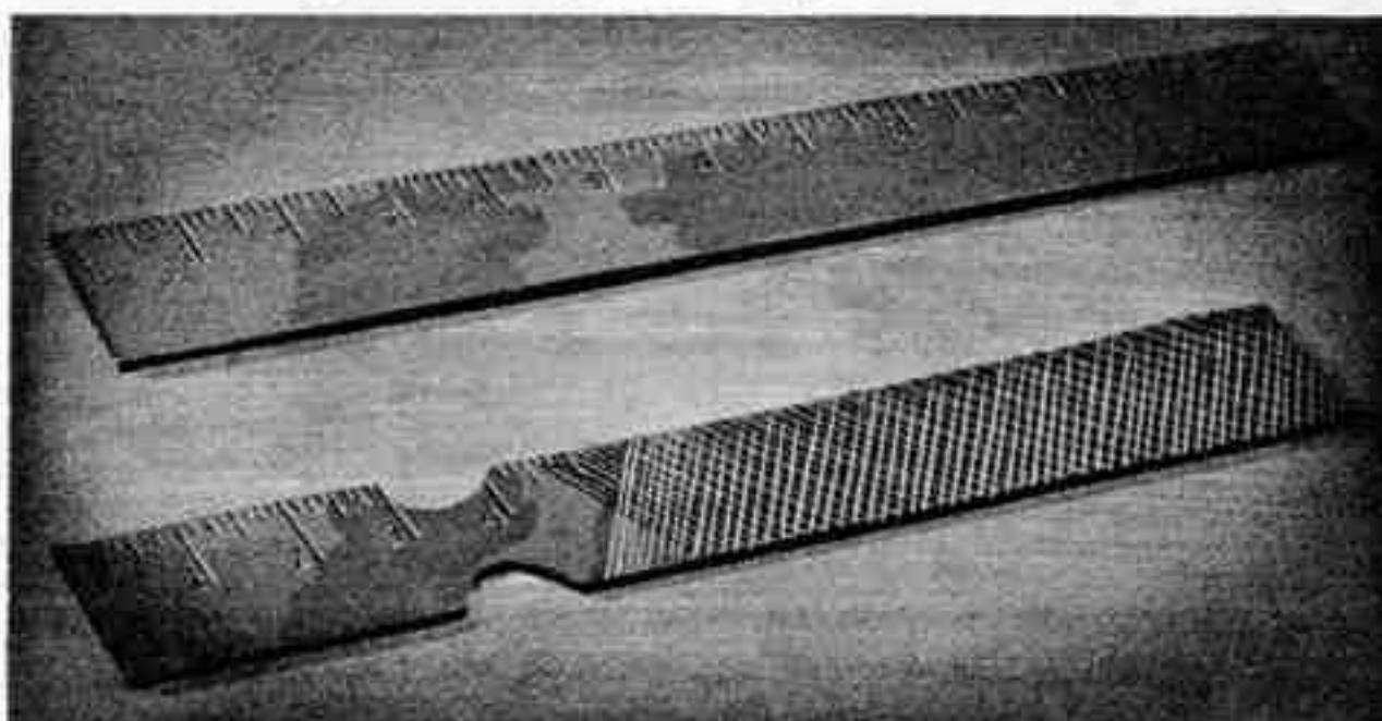
FILE MADE FROM STEEL RULE
